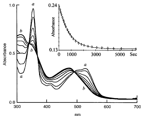
FIGURE 2: Reaction of Cbl(III) with NO as a function of time. Approximately 3 mL of 55 \mu M deoxygenated aqueous hydroxocobalamin was bubbled with high-purity NO gas for 4 min ([NO] = 1946 \mu M). Perchloric acid was added to a final concentration of 0.1 M, and spectra were recorded as a function of time until no further change was observed. At the end of the experiment, Ar was bubbled through the solution for 10 min to remove NO before the pH was measured. On other occasions, NO was added after the acid, with the same results obtained. (a) Spectrum immediately after addition of acid. (b) Spectrum when no further changes were observed. (Inset) Time course at 525 nm for the reaction using 28 \mu M Cbl(III) and 1946 \mu M NO. Diamonds, data points; line, best single-exponential fit.
